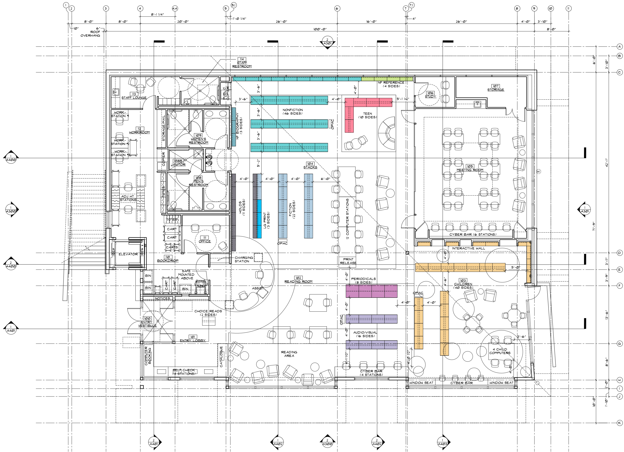
MAIN LEVEL FURNITURE PLAN 1 FOR REFERENCE ONLY. FURNITURE IS OFO
