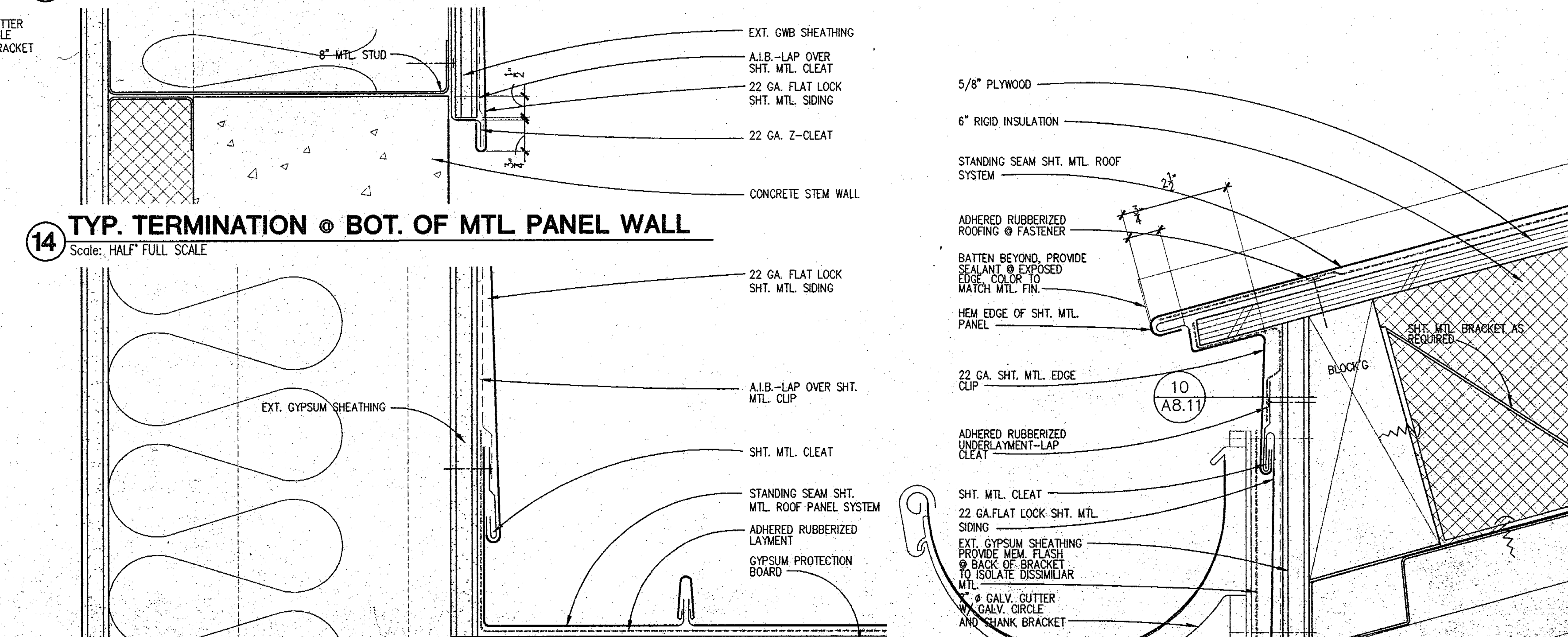
14 TYP. TERMINATION @ BOT. OF MTL PANEL WALL Scale: HALF FULL SCALE
