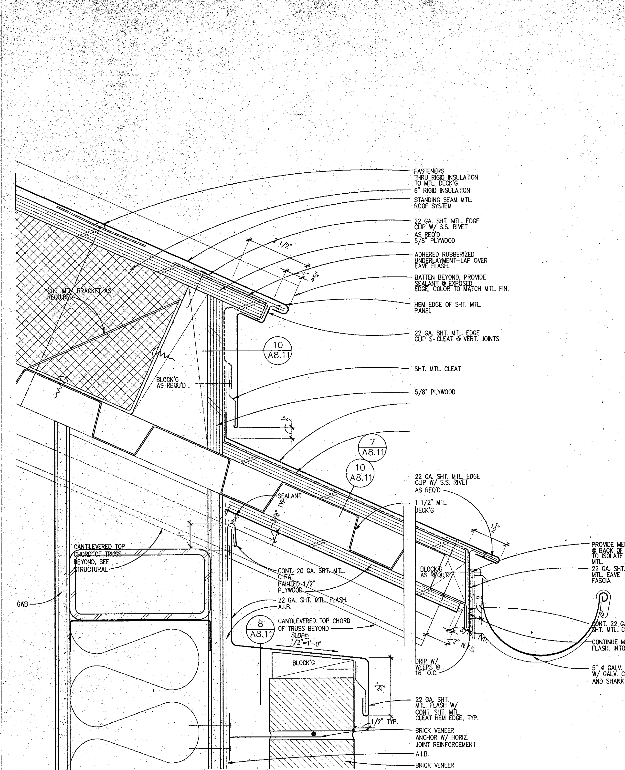
13 TYP. ROOF/EAVE @ TOP OF BRICK VENEER WALL Scale: HALF FULL SCALE
