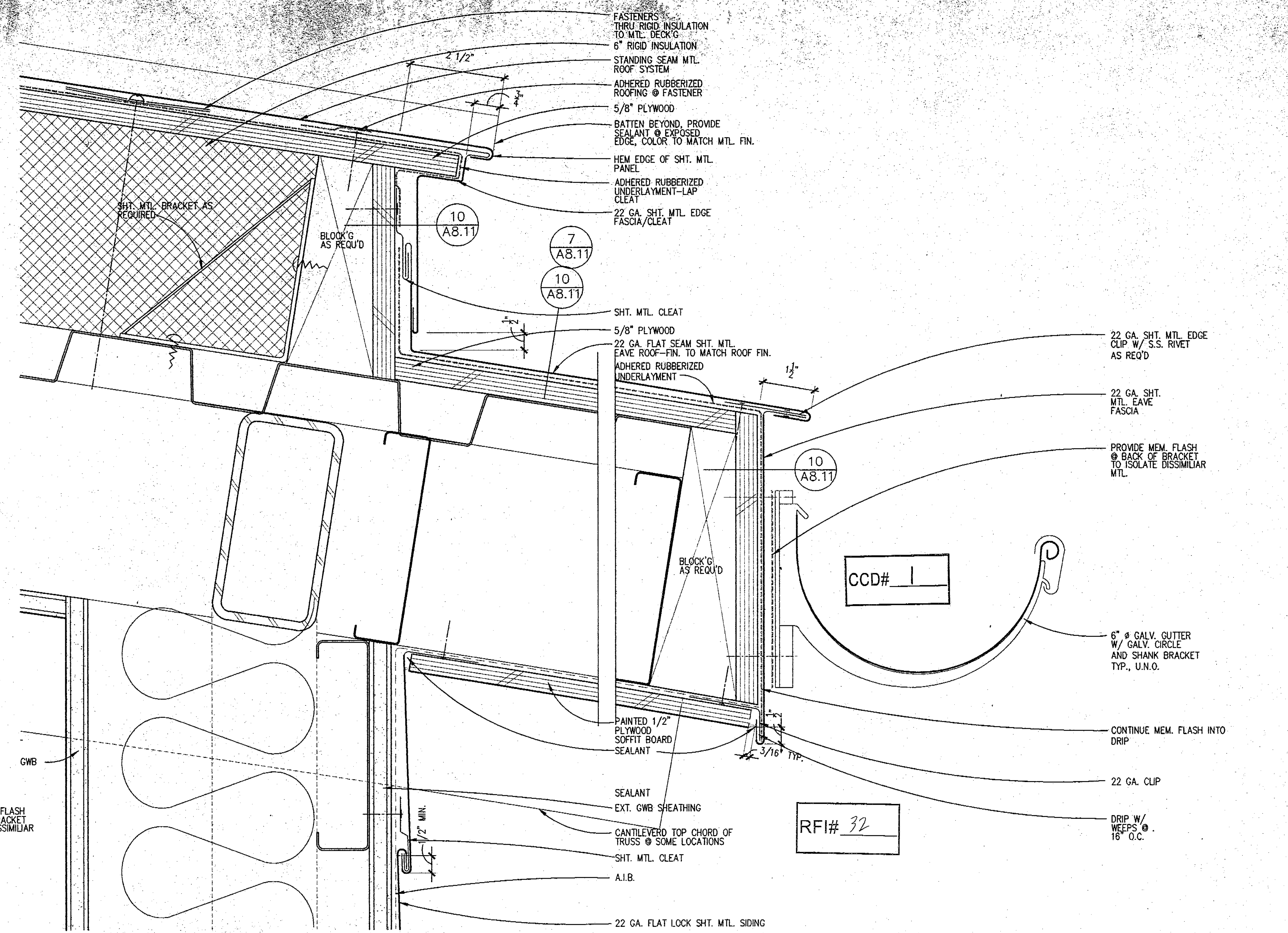
10 TYP. ROOF/EAVE @ TOP OF MTL PANEL WALL Scale: HALF FULL SCALE
